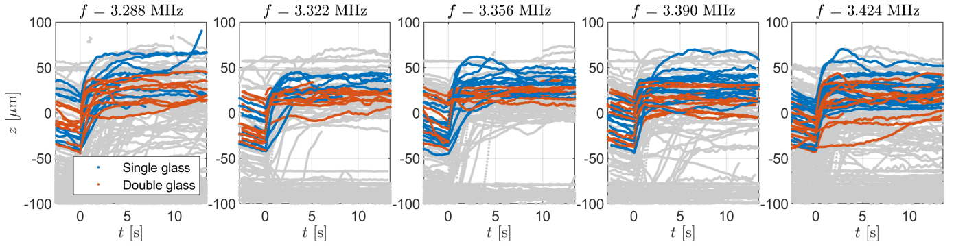
Figure 3. Focusing time for the different frequencies. The PZT transducer is switched on at t = 0 . For t < 0 , the polystyrene spheres sediment with a velocity of approximately 2.9 \mu\text{m/s} . The acoustic energy density is calculated on trajectories with z -position at t = 0 between -45 and 20 \mu\text{m} , highlighted in blue and orange for particles in the single-glass and double-glass zone, respectively.
