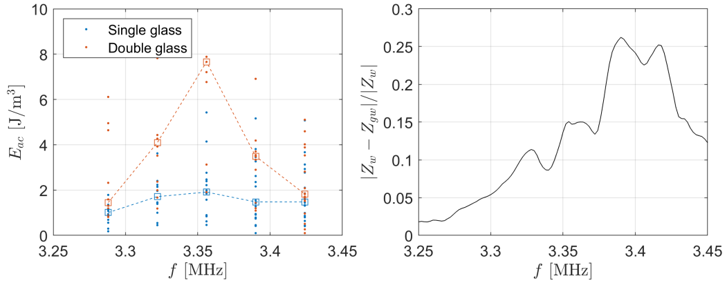
Figure 4. Left: acoustic energy density as a function of the actuation frequency for single-glass and double-glass region. Squared markers represent the median values. Right: Normalized differential impedance spectrum with the channel filled with water and a solution 10%-glycerol/water.
