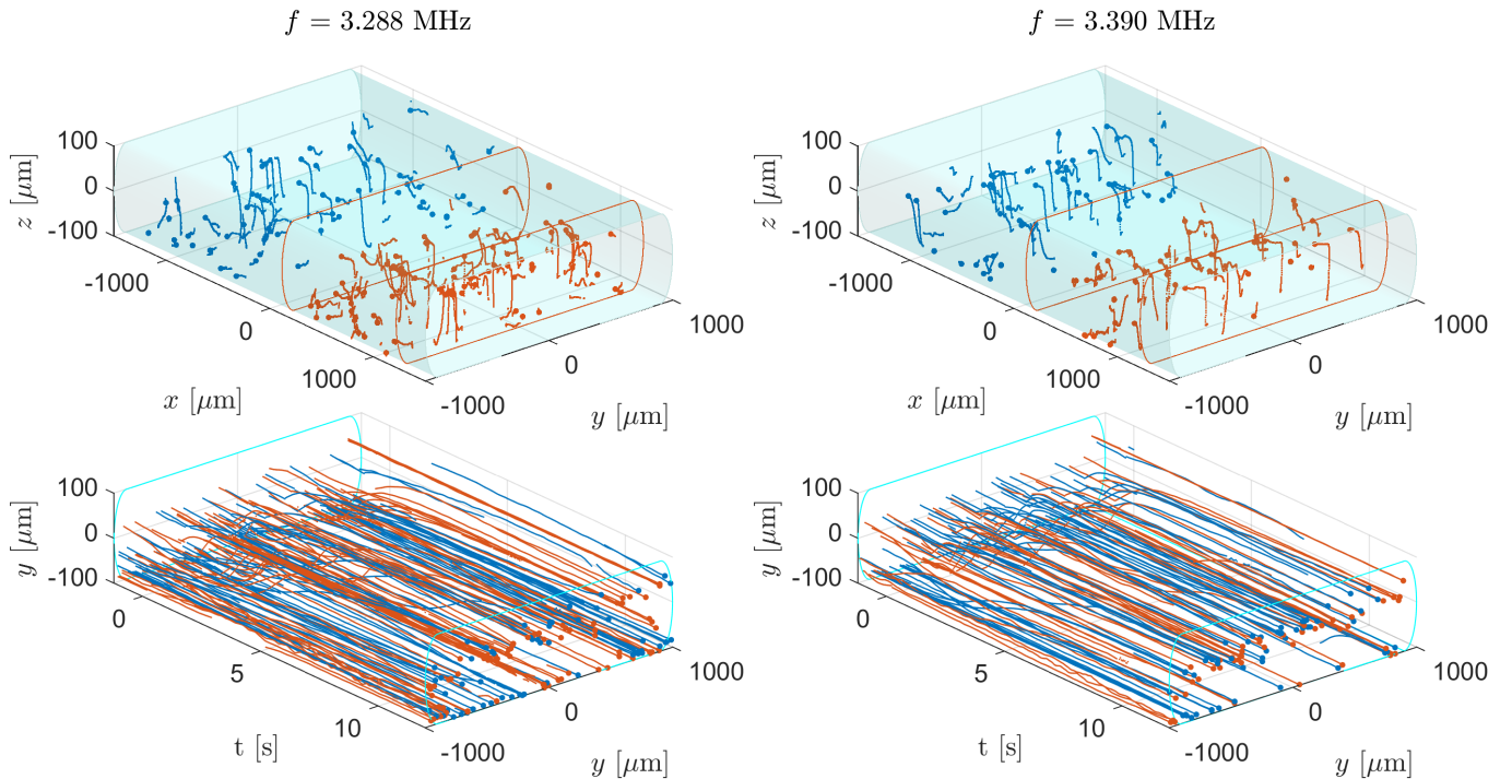
Figure 2. Example of 3D particle trajectories obtained at different frequencies. Top: particles in the measurement volume. Particles in the double-glass region are plotted in orange. Bottom: Cross-sectional particle position as a function of time. After the the ultrasound is switched on the particles move to the nodal plane.
