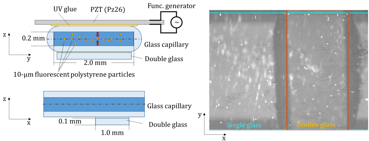
Figure 1. Left: Sketch of the acoustofluidic device consisting of a glass capillary tube with internal cross-section of 2.0 \times 0.2 \text{ mm}^2 . The ultrasound actuation is provided by a piezoelectric transducer glued on the capillary tube. The thickness of the wall is modified locally by gluing a 0.1-mm-thick glass slide. Right: Defocused particle images taken with a 5\times microscope objective with a cylindrical lens in front of the camera sensor. The double-glass region is highlighted in orange.
