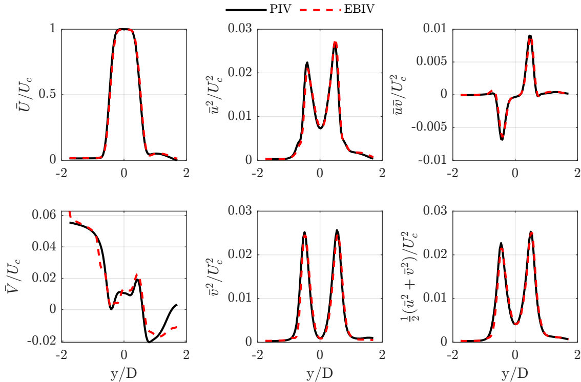
Figure 4. Statistics comparison between the conventional PIV (black line) and the EBIV (dashed red line) cameras results. Statistics are plotted at the longitudinal location x/D = 2 .
